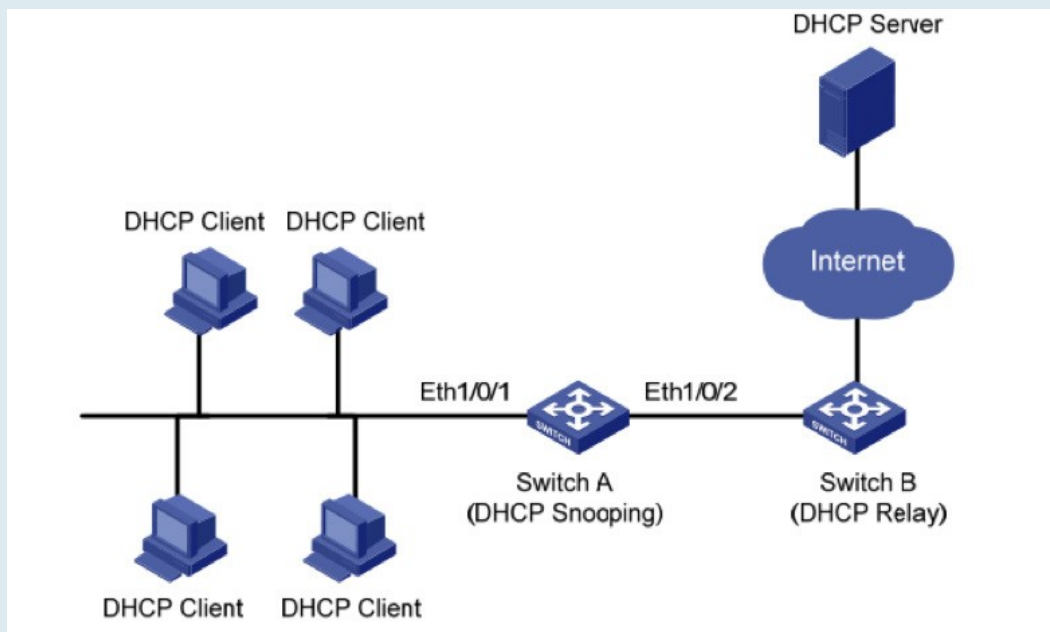
Typical Networking of DHCP Snooping
